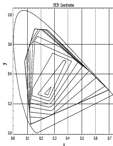
Unconstrained LED Drive Currents. — Shows contours of maximum available luminous intensity as a function of pixel CIE color coordinates (x, y). The heavy black line encloses the gamut. Contours are at {0.95, 0.85, 0.75, ..., 0.05} times the maximum available luminous intensity (I m =11.8 candelas).
