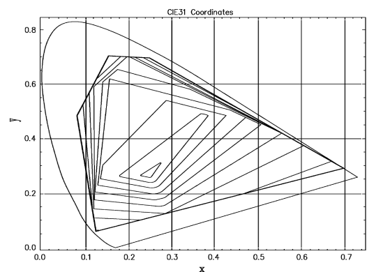
Unconstrained LED Drive Currents. — Shows contours of maximum available luminous intensity as a function of pixel CIE color coordinates (x, y). The heavy black line encloses the gamut. Contours are at {0.95, 0.85, 0.75,...,0.05} times the maximum available luminous intensity ( Y=11.8 candela).
